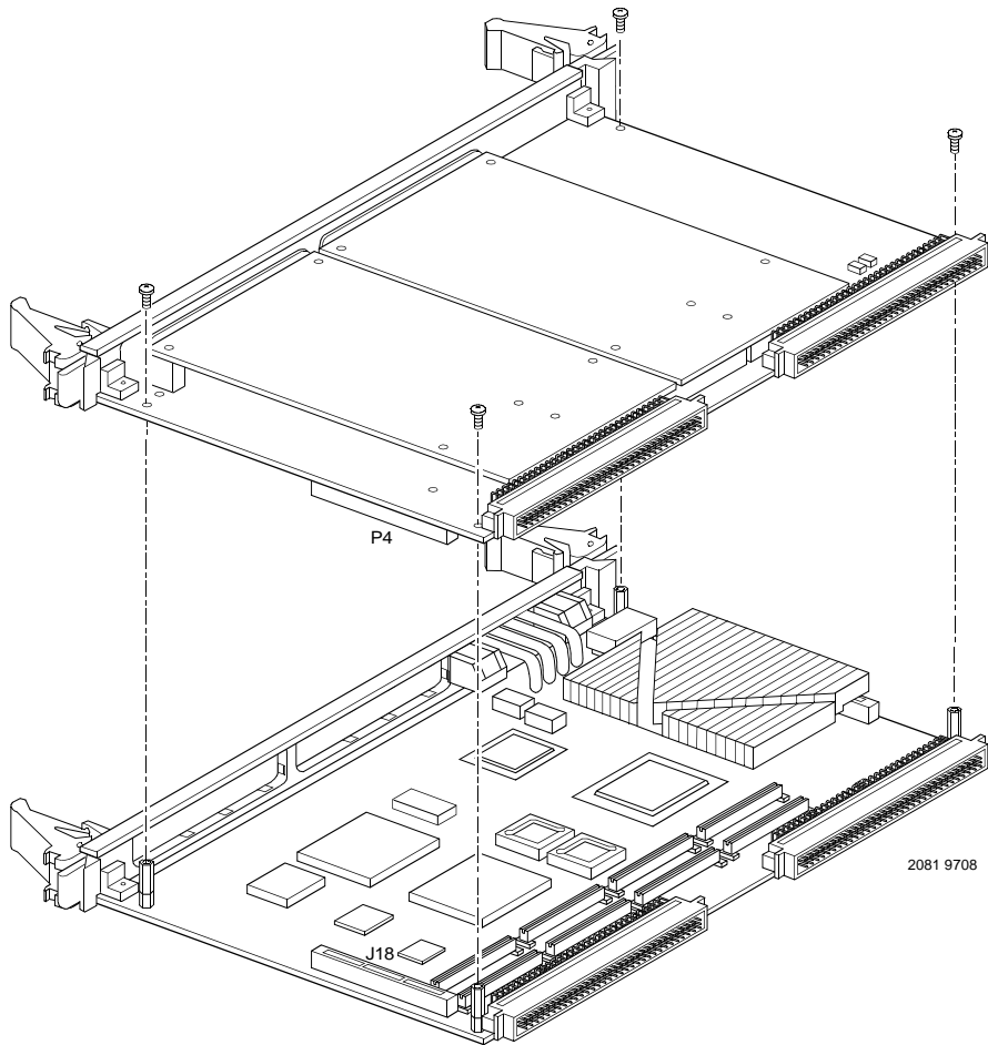
Figure 1-4. PMCspan-002 Installation on an MVME2300
