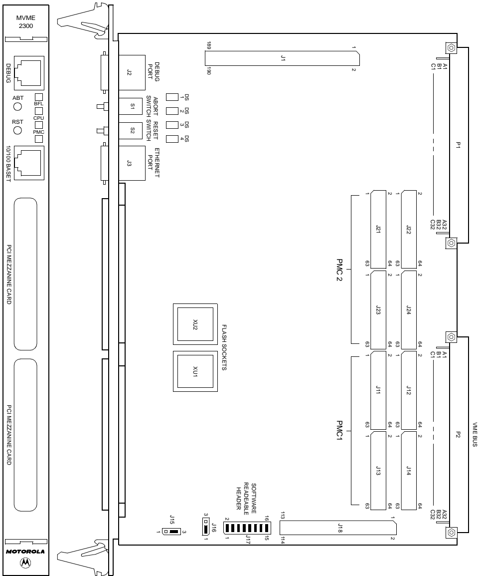
Figure 1-1. MVME2300 Switches, LEDs, Headers, Connectors
